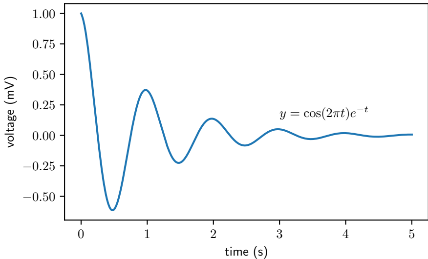
Damped exponential decay
